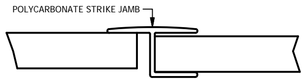
DETAIL C SCALE 1 : 1
