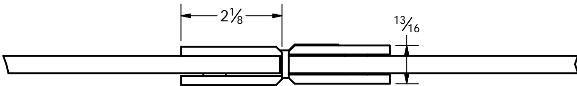
DETAIL B GLASS-TO-GLASS HINGE
