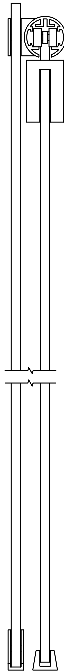
DETAIL @ DOOR
