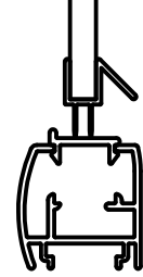
DETAIL @ DOOR
