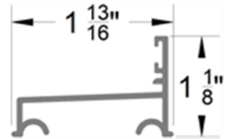
Bypass Bottom Track / Carril inferior de bypass x1
