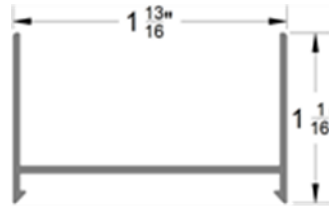
Bypass Wall Jamb / Jamba de bypass x2
